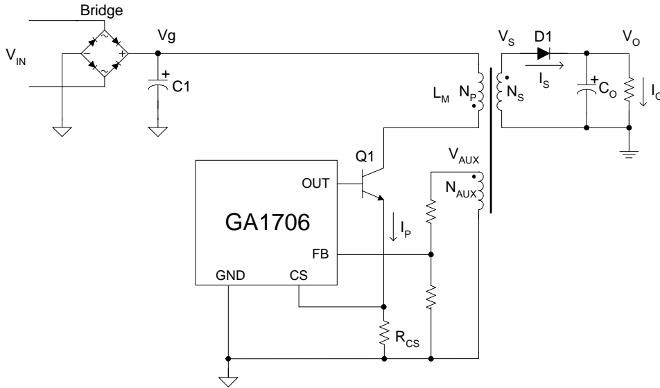
Figure 10. Simplified Flyback Converter Controlled by GA1706
