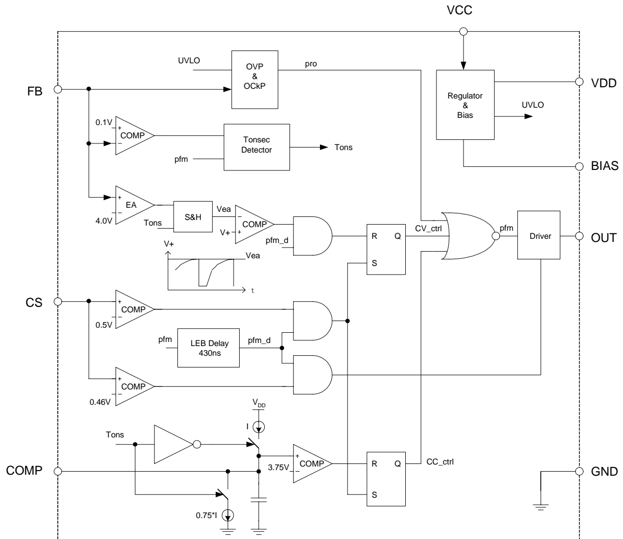
Figure 3. Functional Block Diagram of GA1706
