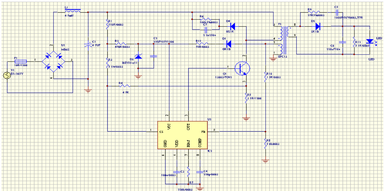
Figure 10. 5V/0.3A Output for LED power
