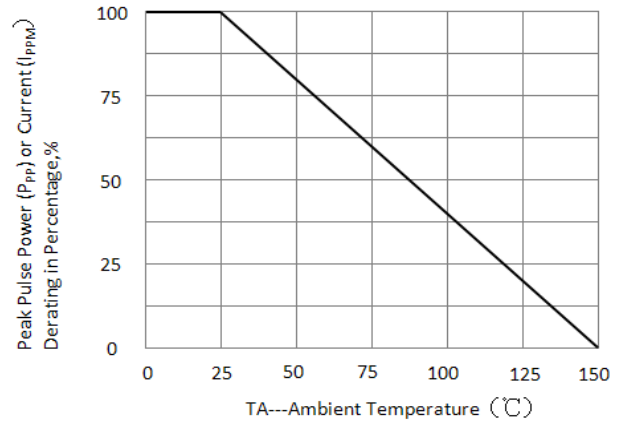
Figure 4. Peak Pulse Power Derating Curve
