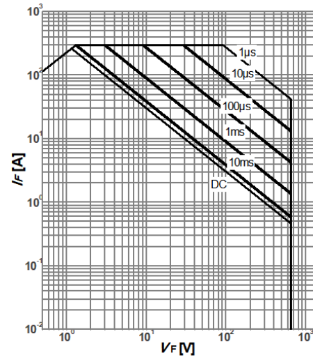
Fig.14 - Diode Safe operating area
