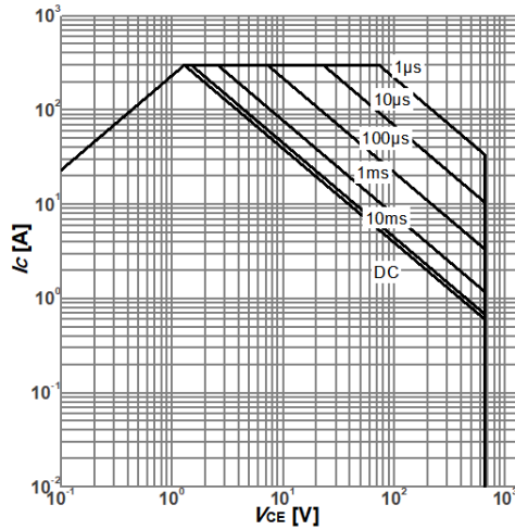
Fig.13 - IGBT Safe operating area
