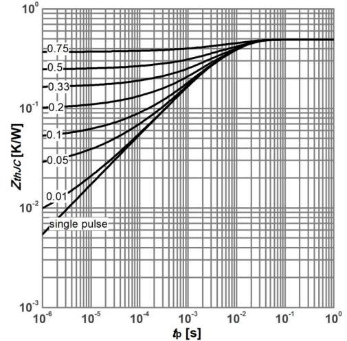
Fig.12 - Diode transient Thermal Impedance, Junction-Case
