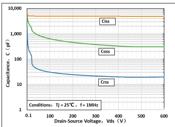
Figure 17: Capacitance Characteristics
