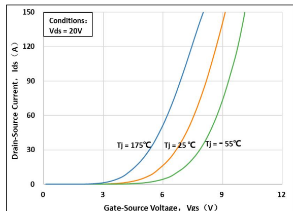
Figure 6. Transfer Characteristic
