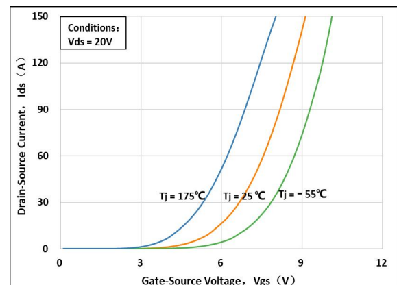
Figure 6. Transfer Characteristic
