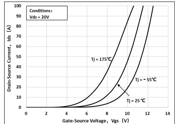
Figure 6. Transfer Characteristic
