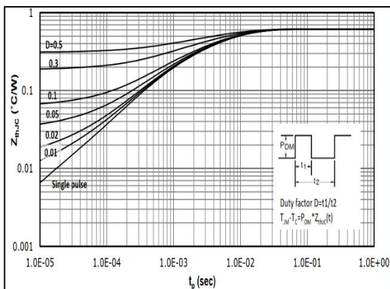
Figure 17: Transient Thermal Impedance
