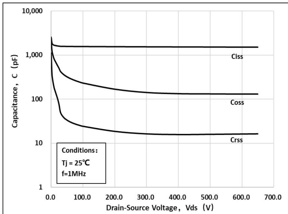
Figure 15: Capacitance Characteristic
