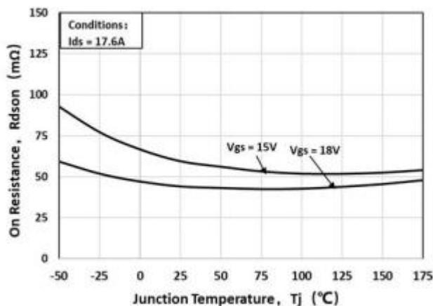
Figure 5. R_{DS(on)} vs. Temperature
