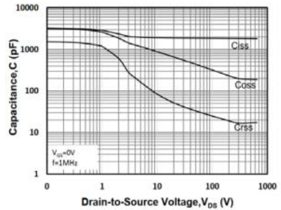
Figure 12: Capacitance Characteristics
