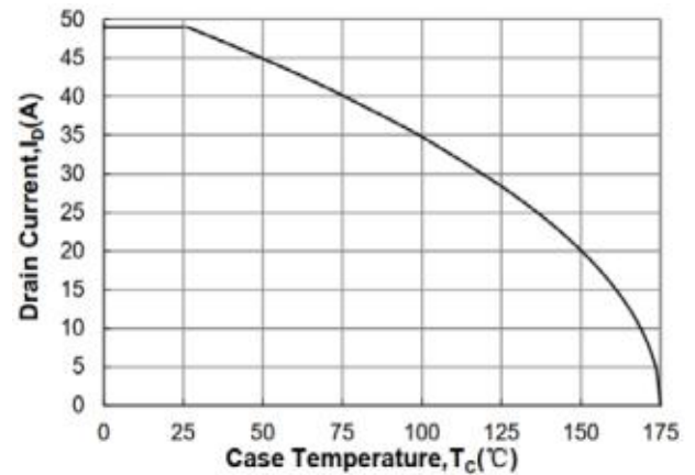
Figure 10: Drain Current vs. Case Temperature
