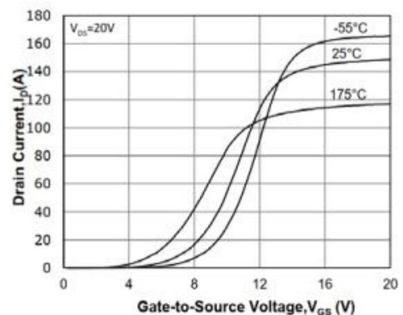
Figure 6. Transfer Characteristic
