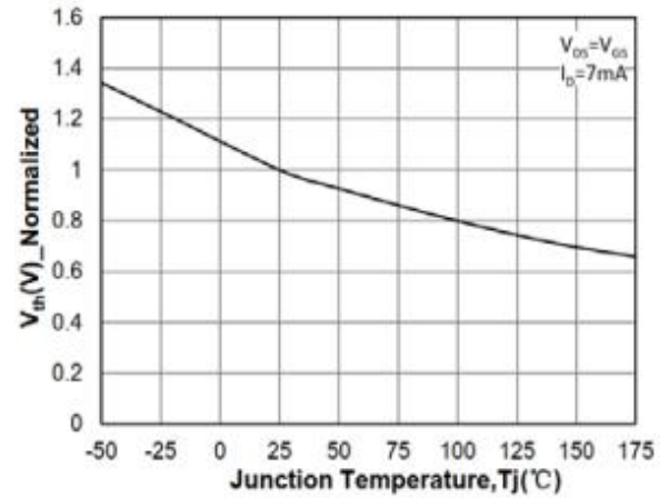
Figure 8: V_{th} Vs T_J Temperature Characteristic
