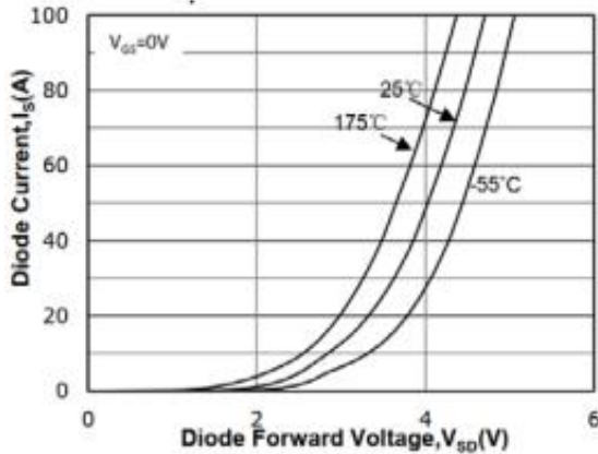
Figure 7: Body-diode Characteristic
