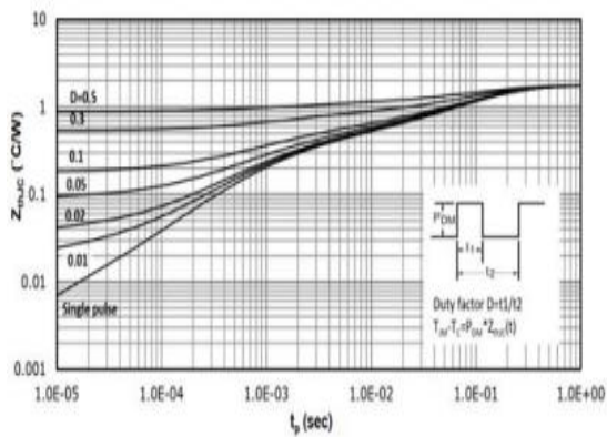
Figure 13: Transient Thermal Impedance
