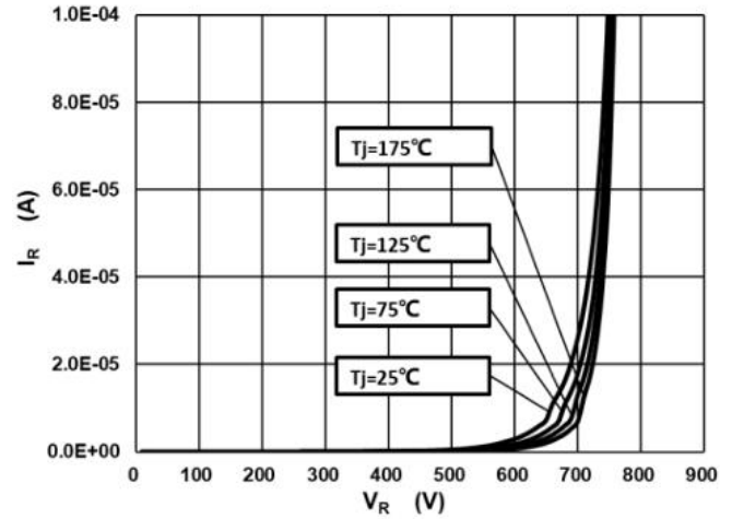
Fig.2 –Reverse Characteristics
