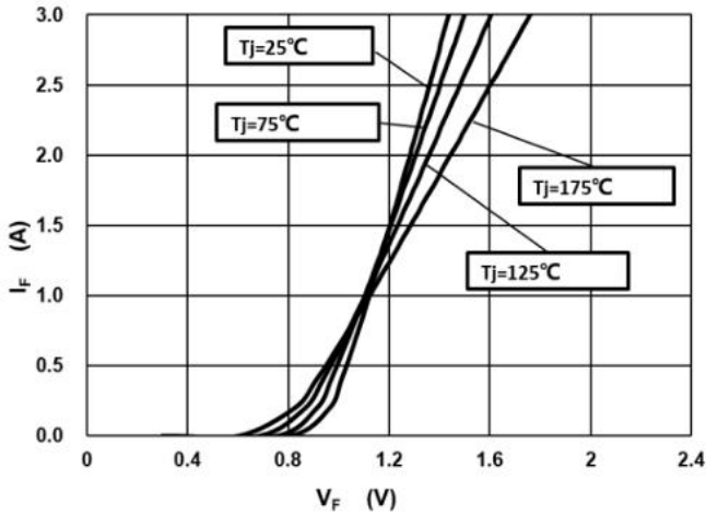
Fig.1 –Forward Characteristics
