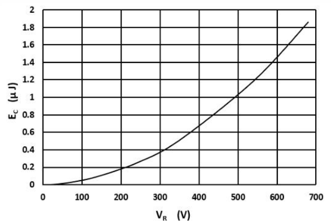
Fig.6 –Typical Capacitance Stored Energy
