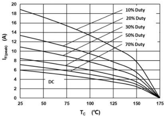
Fig.3 –Current Derating
