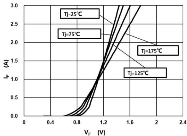
Fig.1 –Forward Characteristics
