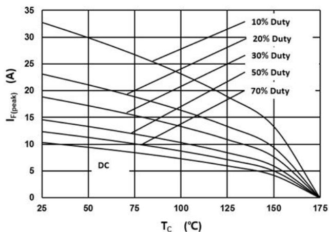
Fig.3 –Current Derating
