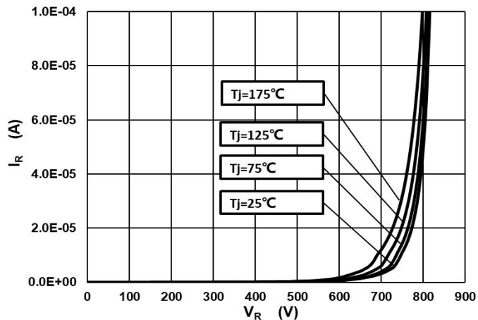
Fig.2 –Reverse Characteristics
