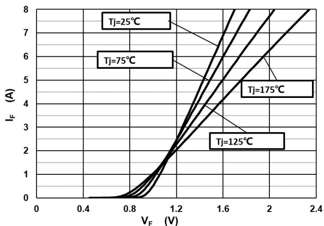
Fig.1 –Forward Characteristics
