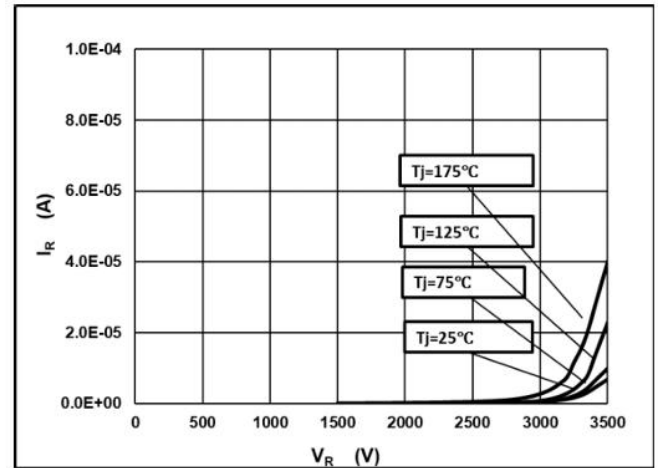
Fig.2 –Reverse Characteristics
