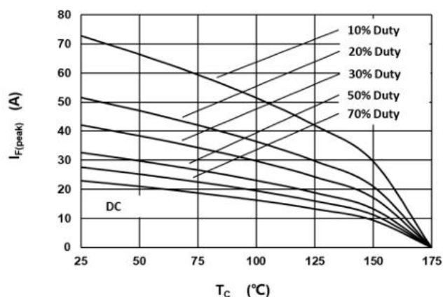
Fig.3 –Current Derating
