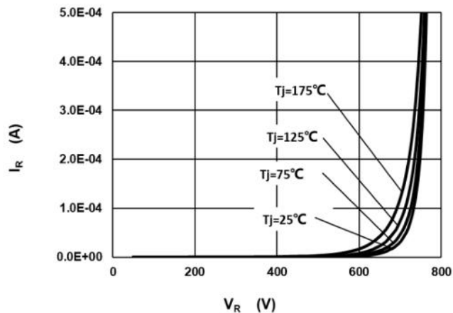
Fig.2 –Reverse Characteristics
