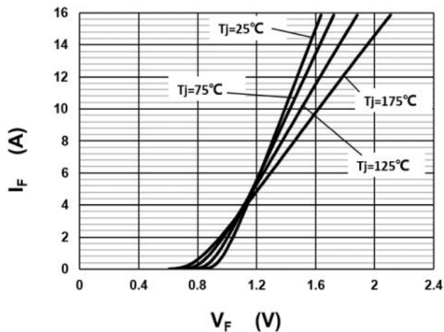
Fig.1 –Forward Characteristics
