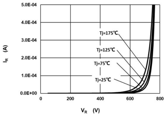
Fig.2 –Reverse Characteristics
