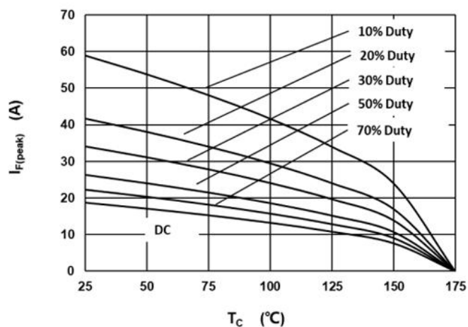
Fig.3 –Current Derating
