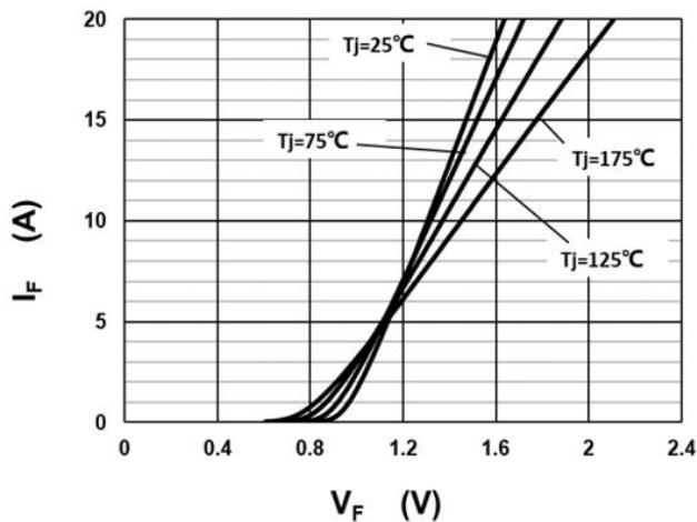
Fig.1 –Forward Characteristics
