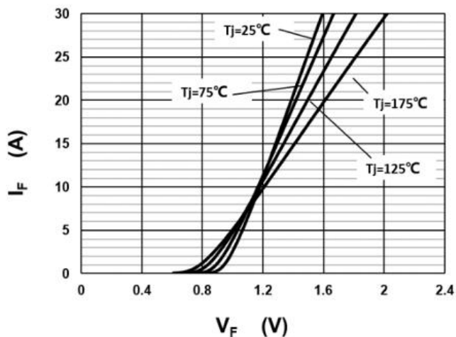
Fig.1 –Forward Characteristics
