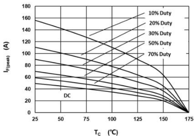
Fig.3 –Current Derating
