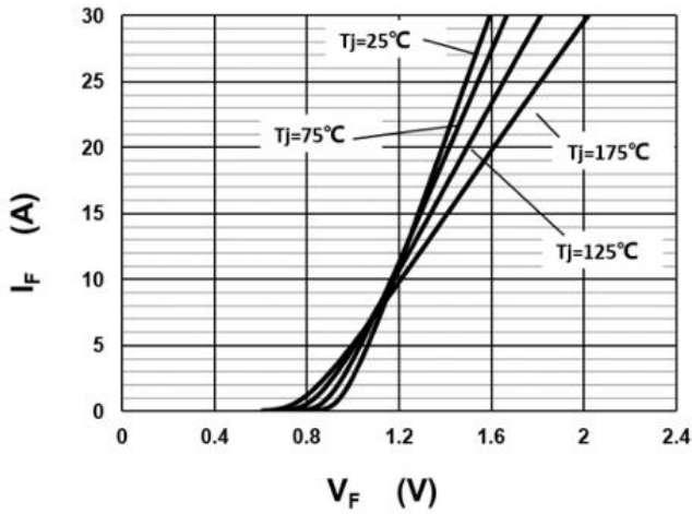
Fig.1 –Forward Characteristics
