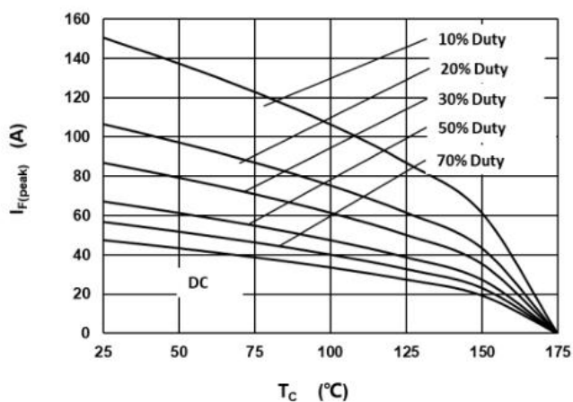
Fig.3 –Current Derating
