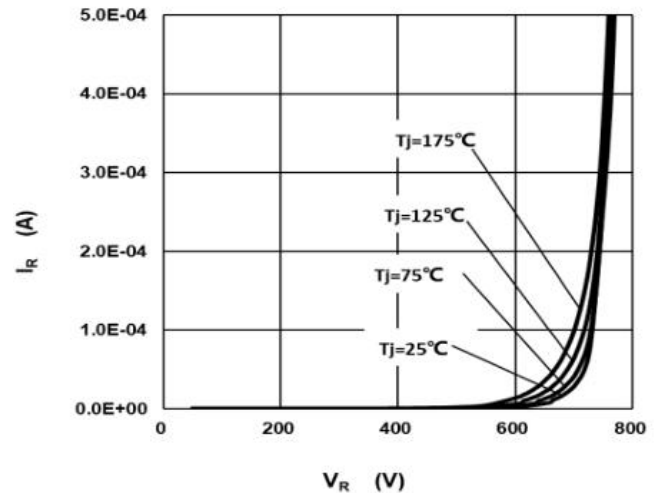
Fig.2 –Reverse Characteristics
