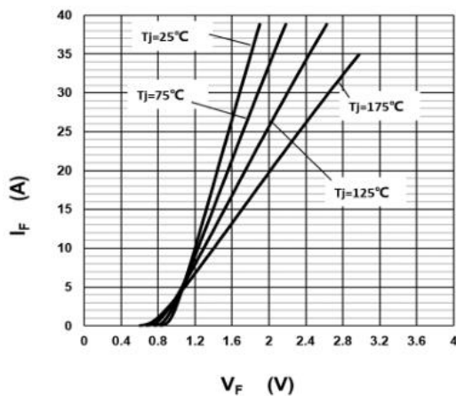
Fig.1 –Forward Characteristics
