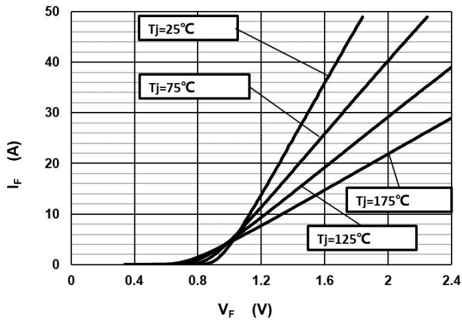
Fig.1 -Forward Characteristics
