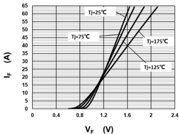
Fig.1 –Forward Characteristics
