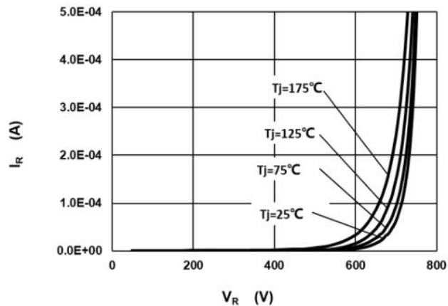
Fig.2 –Reverse Characteristics
