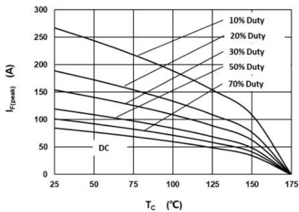
Fig.3 –Current Derating
