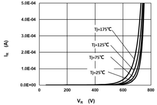
Fig.2 –Reverse Characteristics
