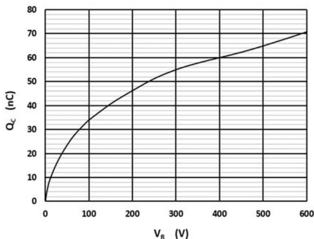
Fig.5 –Total Capacitance Charge vs. Reverse Voltage
