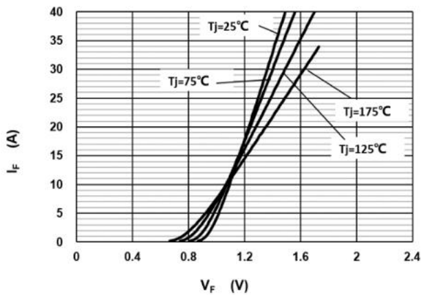
Fig.1 –Forward Characteristics
