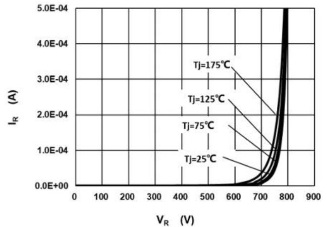
Fig.2 –Reverse Characteristics
