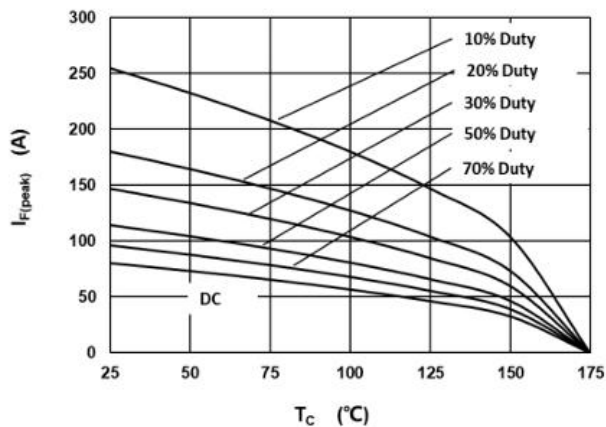
Fig.3 –Current Derating
