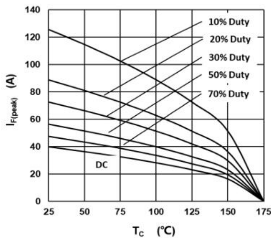
Fig.3 –Current Derating
