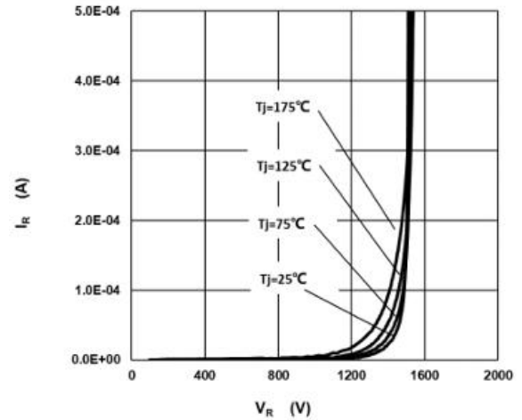
Fig.2 –Reverse Characteristics
