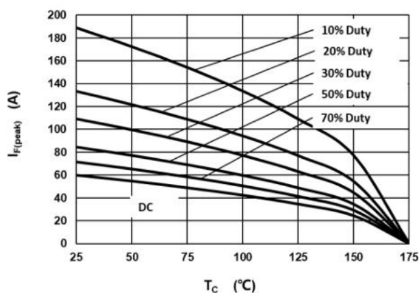
Fig.3 –Current Derating
