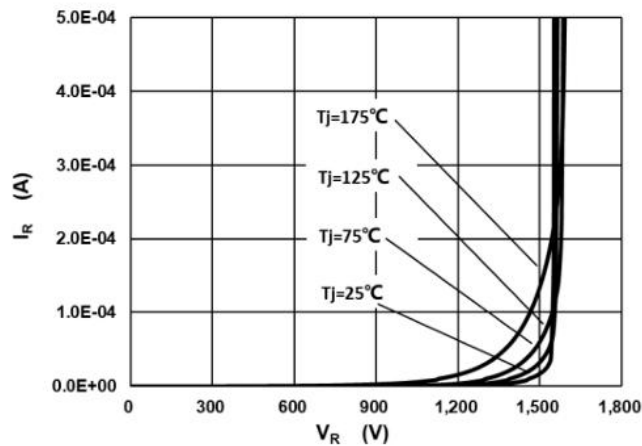
Fig.2 –Reverse Characteristics
