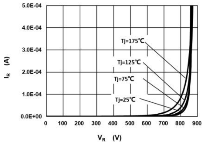
Fig.2 –Reverse Characteristics
