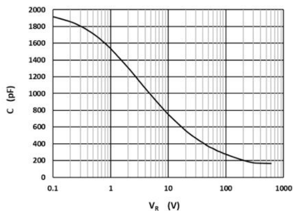
Fig.2 –Reverse Characteristics
