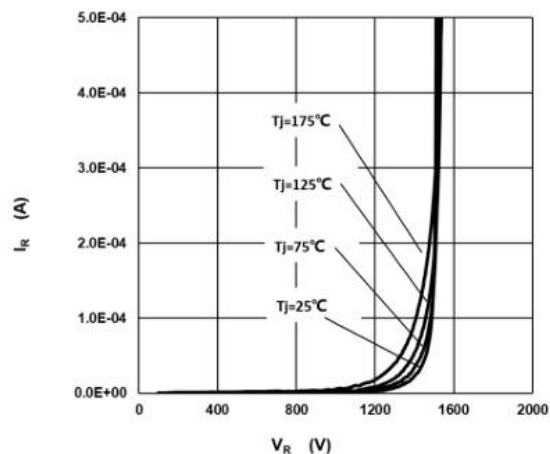
Fig.2 –Reverse Characteristics
