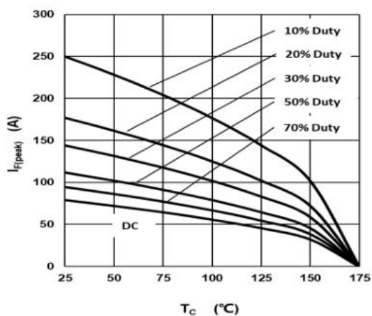
Fig.3 –Current Derating
