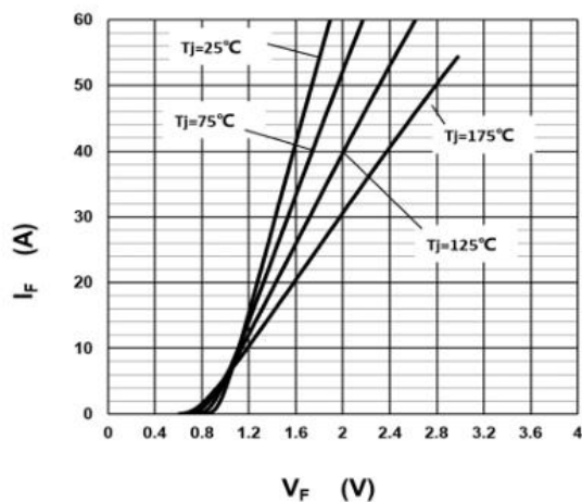
Fig.1 –Forward Characteristics
